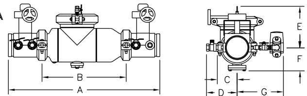
MODEL 350ASTDA with BGVIC option
